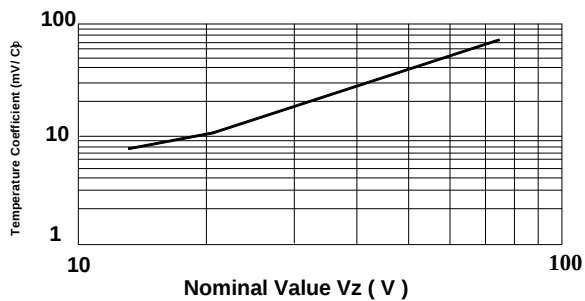
Temperature Coefficient
