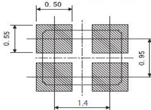
Example of a Terminal Land Pattern
