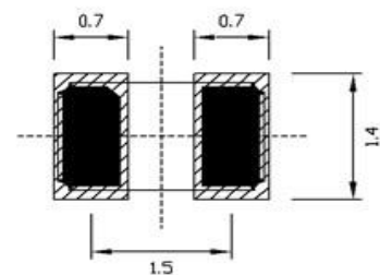
LAND PATTERN (REFERENCE)
