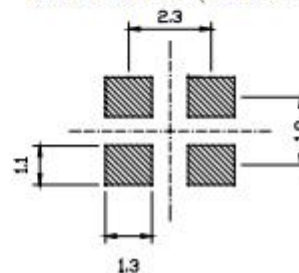
LAND PATTERN (REFERENCE)
